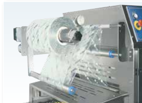
Svolgitore elettronico proporzionale. Self-adjusting electronic unwinding system with encoder. Déroulement électronique proportionnel. Desbobinador electrónico proporcional.
